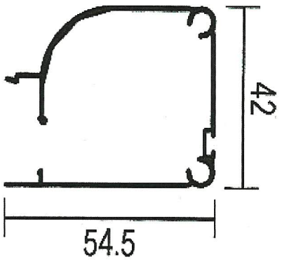
DETAIL BOVENBAK / DETAIL PROFILE CAISSON
